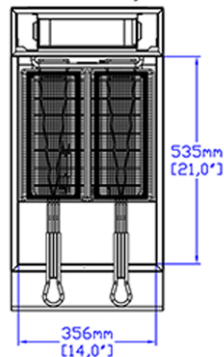
3 tube Fryer
